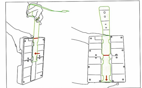
Position the attachment on the line and slide it down to the stop.
