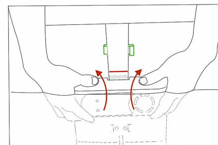
Position the top of Sensor Espio™ opposite the mark on the attachment support. Slide it upwards on the attachment support.
