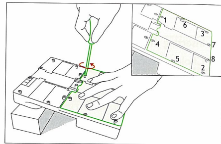
In order to ensure waterproofing, screw in the tightening sequence given.
