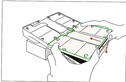
Place Sensor Espio™ on a prop, as shown. Unscrew the battery compartment screws.
