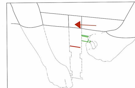
You must insert the shim supplied 2 in above the mark, between the wall of the pool and the attachment support.
