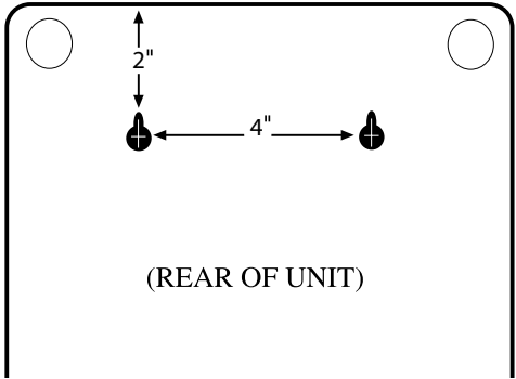
Figure 2-1. Wall Mount
